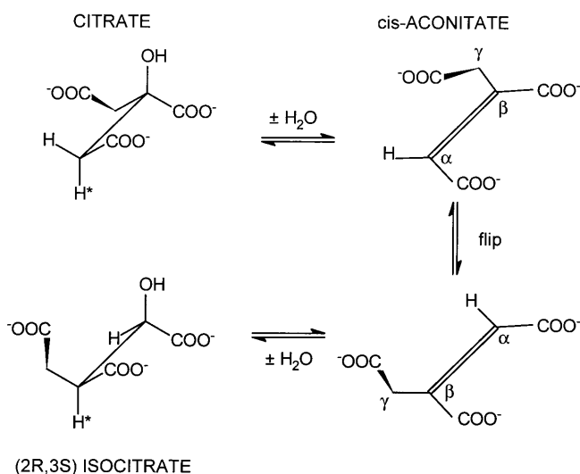
FIG. 3. Proposed mechanism for the reactions catalyzed by aconitase. The “flip” step indicates that cis -aconitate must be released (displaced) and rebound in the alternate binding mode.
